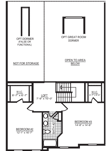
UPPER LEVEL ELEVATION C
