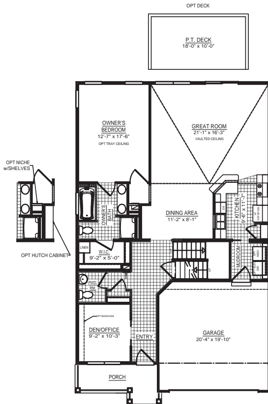
MAIN LEVEL ELEVATION C
