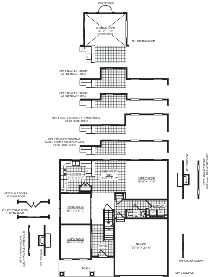
MAIN LEVEL ELEVATION C
