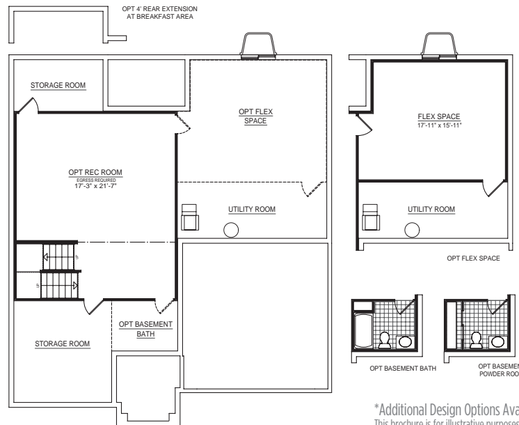
LOWER LEVEL ELEVATION C
