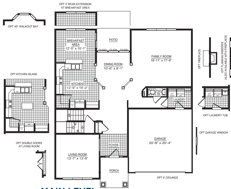
MAIN LEVEL ELEVATION C
