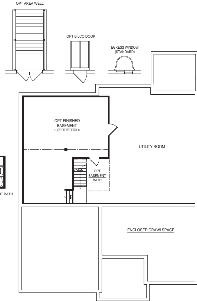
LOWER LEVEL ELEVATION A
