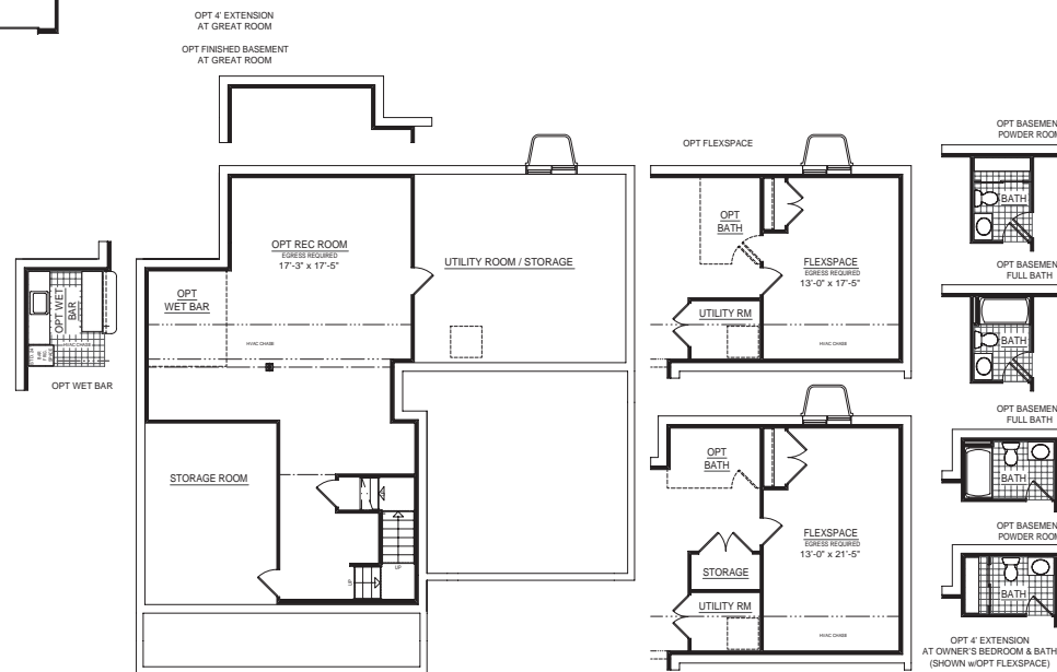
LOWER LEVEL ELEVATION C
